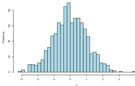
Histogram of a Standard Normal Random Variable
